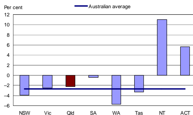
Figure 1: Monthly change in total dwelling units approved (trend), June 2010
